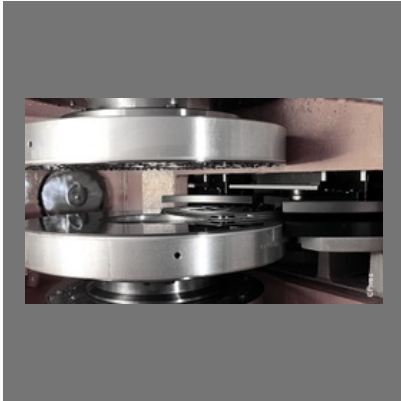
Double Disc Grinding Machine
